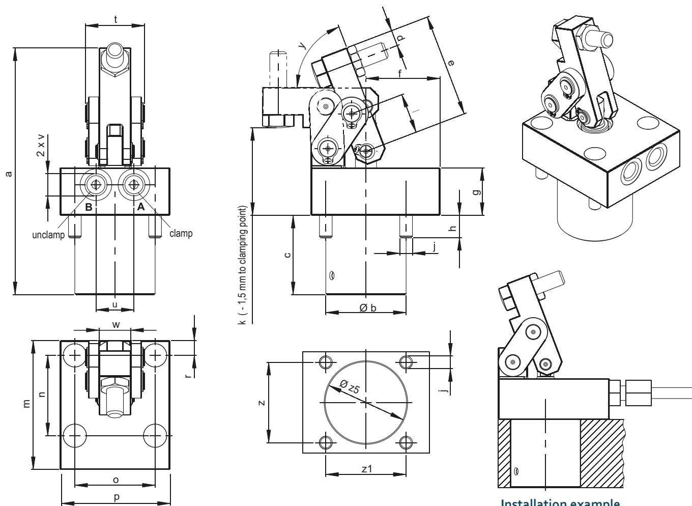
Installation example
