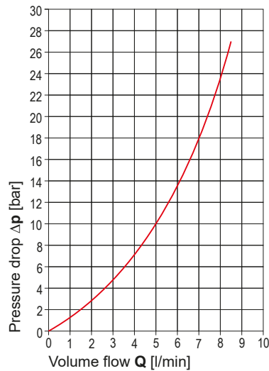
\Delta p -Q nominal line for kinematic viscosity of 53 \times 10^{-6} \text{ m}^2/\text{s} (HLP 22 at 20^\circ \text{C} )
